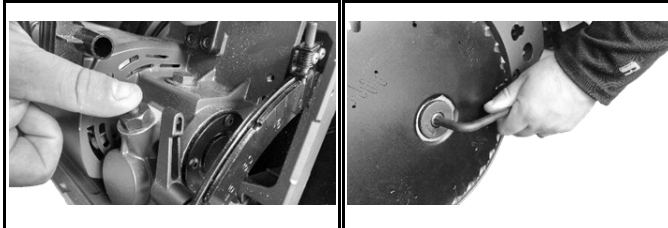
Figures 10a and b. Depress blade lock button while using bolt wrench. Arbor bolt wrench is stored round sleeve above thumb in left image. Turn wrench clockwise to loosen.
