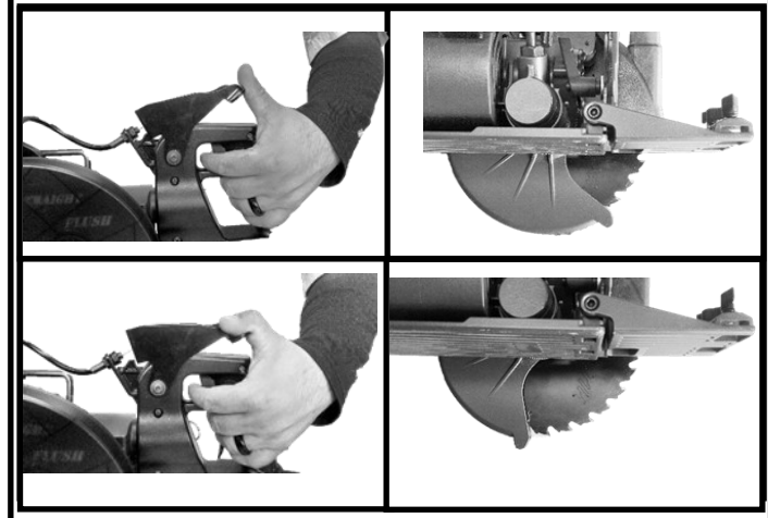
Figures 3a - c. Retracting the lower guard.
