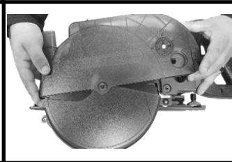
Figures 9a and b. Dust cover removal after releasing magnet on dust cover.
