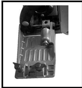
Figures 4a and b. Base Extension Plate (extended and retracted).
