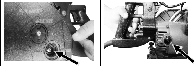
Figures xxa and b. Carbon brushes are located on either side of saw and accessible by removing the black caps.
