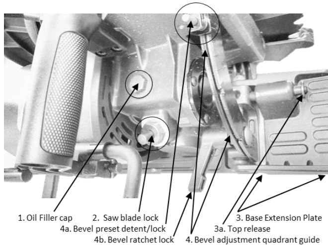
Figure x. Left side of saw.
