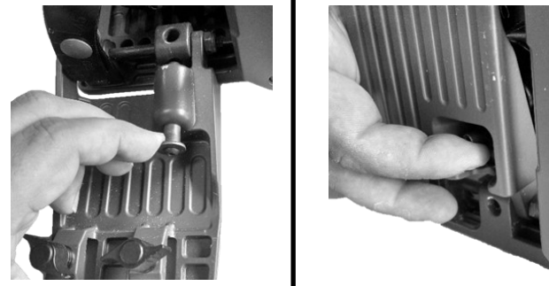
Figures 5a and b. Base Extension Plate (resetting the plate).
