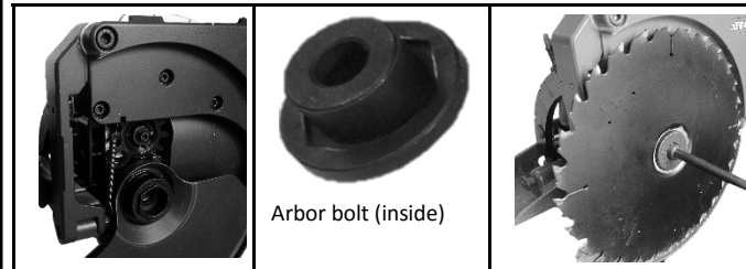
Figures 11a - c. Arbor without blade (lower guard spring to upper left of arbor), bolt and replaced blade. Blade must be securely fitted to arbor. Lock blade and turn counter-clockwise to seat arbor and secure blade.
