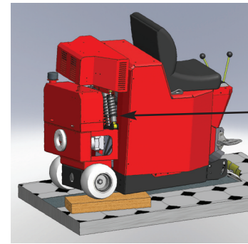
Suspension Cylinders
