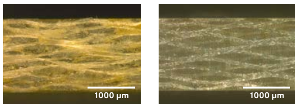
Cut edges of milled (left) and laser-cut (right) FR4 material. Clearly visible: After the milling process, the edge shows open structures with fraying; laser cutting generates a closed surface.
