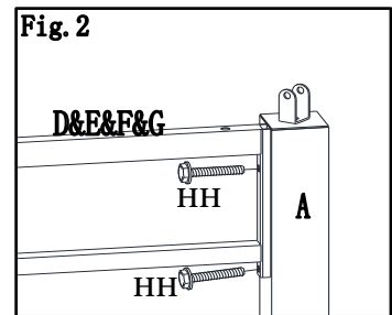
Fig.2: By using bolt(HH) fix screen to post(A).
