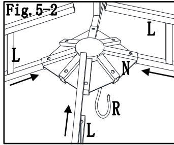
Fig.5-2: Insert slanting beam upper end(L) into large top connector(N),then attach hook(R) to top connector(N).
