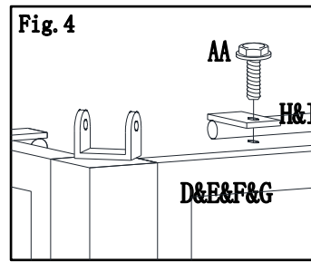
Fig.4: Attach long netting rod(H) to long screen, short netting rod(I) to short screen, by using bolt(AA).
