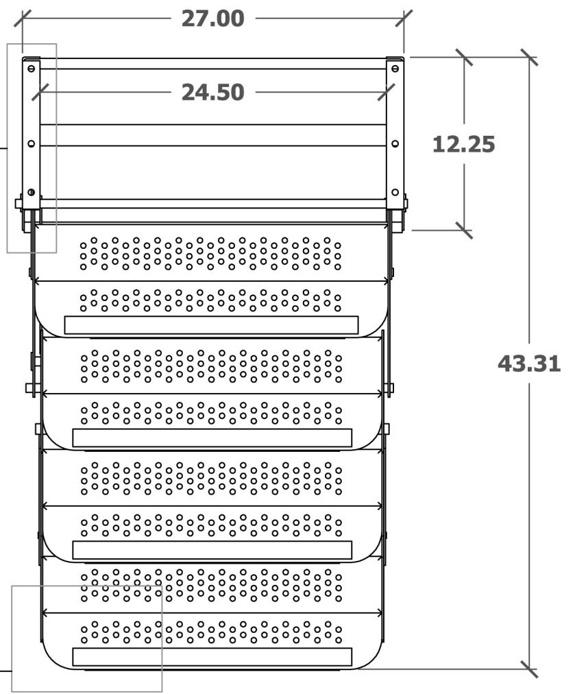
Top View No Scale
