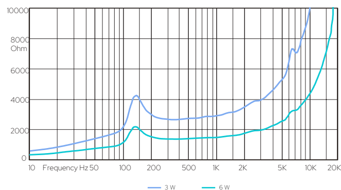
Impedance
