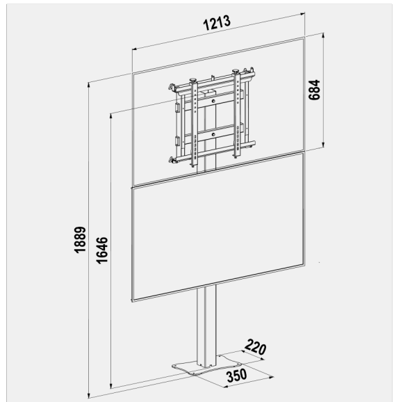
STANDYALL-H 2X1 cod. 08014 Single Side cod. 08020 Back to Back
