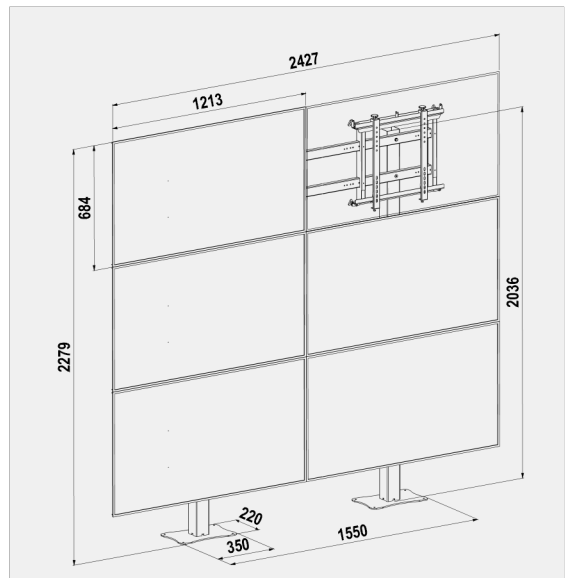
STANDYALL-H 3X2 cod. 08015 Single Side cod. 08018 Back to Back
