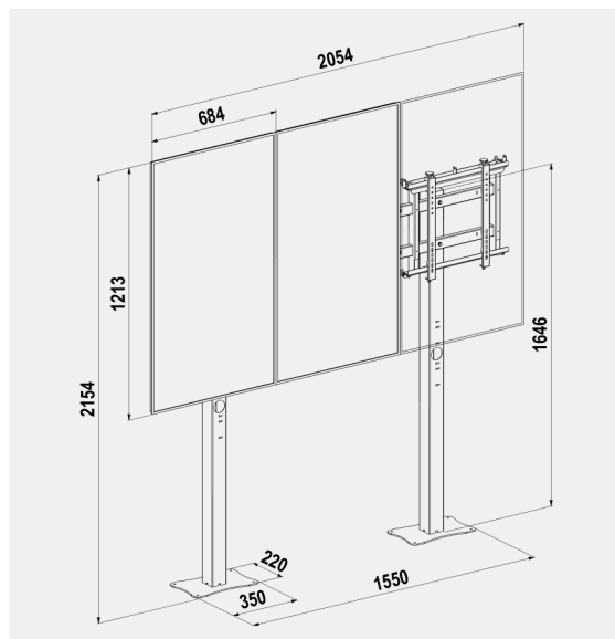
STANDYALL-V 1X3 cod. 08032 Single Side
