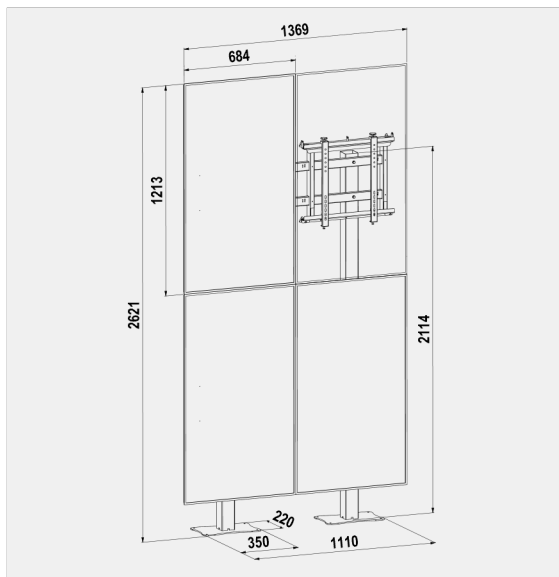
STANDYALL-V 2X2 cod. 08033 Single Side
