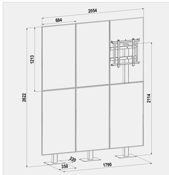
STANDYALL-V 2X3 cod. 08034 Single Side
