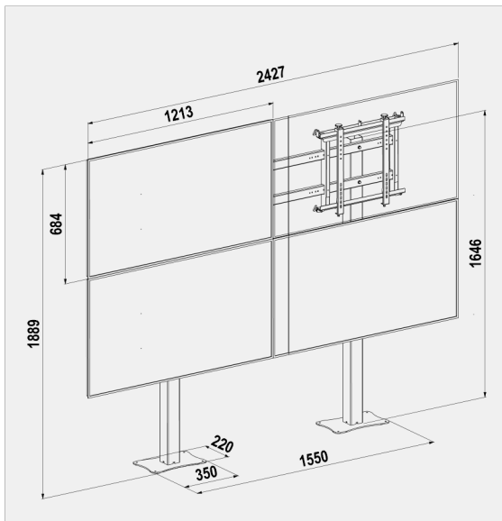
STANDYALL-H 2X2 cod. 07096 Single Side cod. 08019 Back to Back
