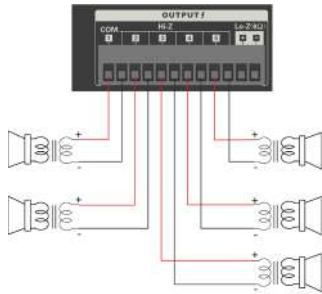
Hi impedance output
