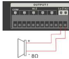
Low impedance output
