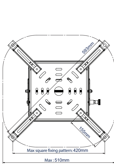
BOTTOM VIEW WITH INCLUDED SHORT EXTENSION LEGS
