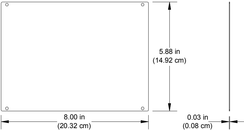
Cover Plate
