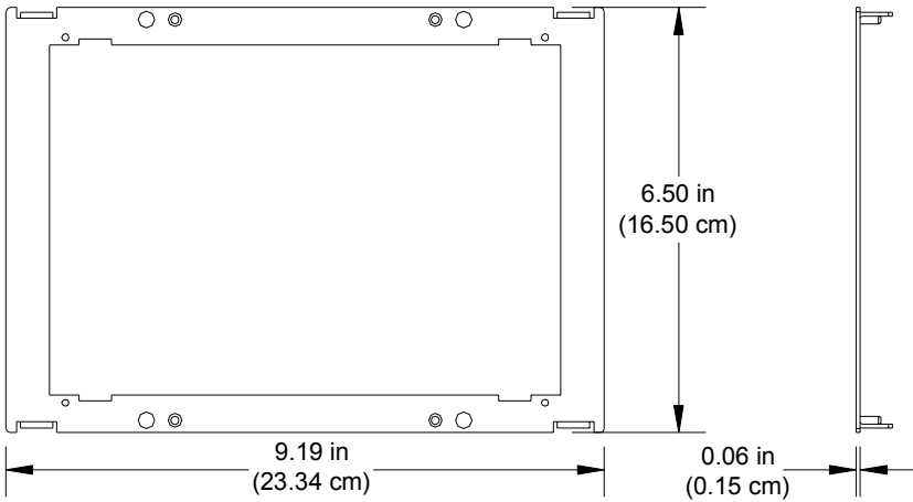
Mounting Plate
