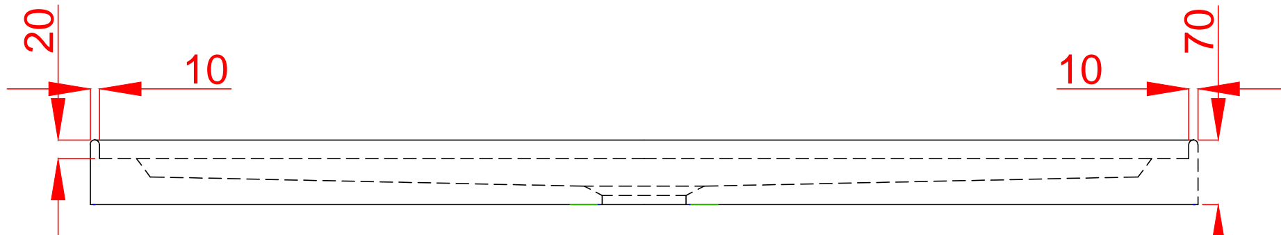
Typical Cross section of a Shower Tray
