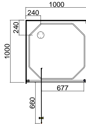
Door opening approx 495mm
