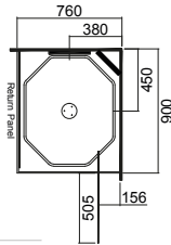
900 x 760 (900 door) (Left Hand Moulding)
