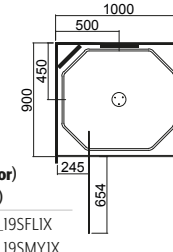
1000 x 900 (1000 door) (Right Hand Moulding)
