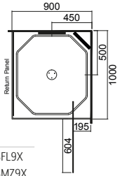
1000 x 900 (1000 door) (Left Hand Moulding)
