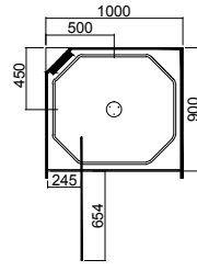
900 x 1000 (1000 Door) (Left Hand Moulding)
