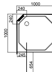
1000 x 1000 (Left Hand Moulding)
