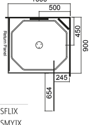
1000 x 900 (1000 door) (Right Hand Moulding)
