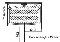
SHOWER OVER 2 SIDED FLAT WALL 0B20002F MOULDED WALL 0B20002M
