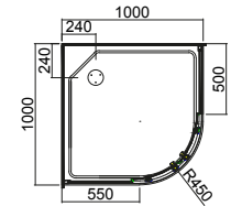
Door opening approx 495mm
