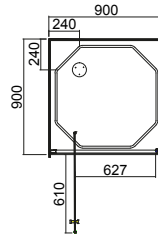
900 x 900 FLAT WALL IPAIW99SFL9C
