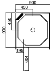
900 x 900 (Left Hand Moulding)
