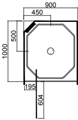
1000 x 900 (900 Door) (Left Hand Moulding)
