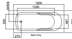
Height with optional upstand 505 mm
