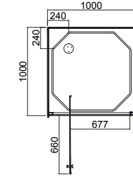
1000 x 1000 FLAT WALL IPAIWIIIIFLIC
