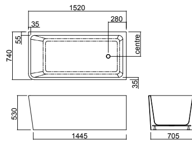
1520 BATH RIGHT HAND NO UPSTANDS 0154000004 WITH UPSTANDS 0154000004U
