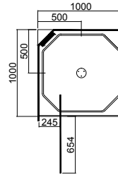
1000 x 1000 (Left Hand Moulding)
