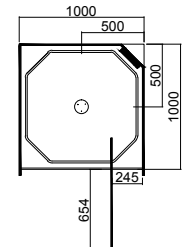
900 x 1000 (1000 Door) (Right Hand Moulding)
