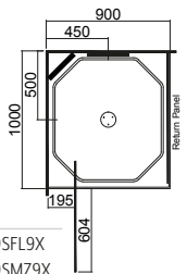
1000 x 900 (900 door) (Left Hand Moulding)
