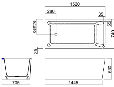
1520 BATH LEFT HAND NO UPSTANDS 0154000003 WITH UPSTANDS 0154000003U
