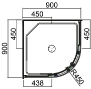
Door opening approx 495mm
