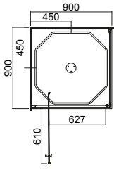
900 x 900 FLAT WALL IPAIW99SFL9X
