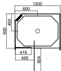
1200 x 900 (Left Hand Moulding)
