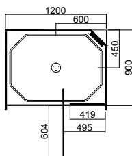
1200 x 900 (Right Hand Moulding)
