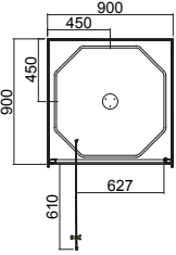
900 x 900 FLAT WALL IPAIW999FL9X
