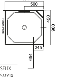
1000 x 900 (1000 door) (Right Hand Moulding)
