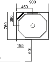
900 x 760 (900 door) (Left Hand Moulding)
