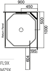
1000 x 900 (1000 door) (Left Hand Moulding)
