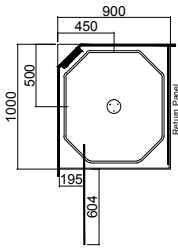
1000 x 900 (900 Door) (Left Hand Moulding)
