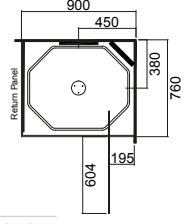
900 x 760 (900 door) (Right Hand Moulding)
