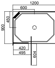
1200 x 900 (Left Hand Moulding)
