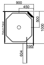
1000 x 900 (900 Door) (Right Hand Moulding)
