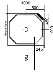
1000 x 900 (1000 Door) (Right Hand Moulding)
