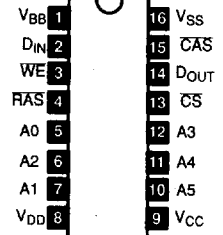
NTE2104 16-Lead DIP, See Diag. 249 NMOS, 4K Dynamic RAM (DRAM), 200ns
