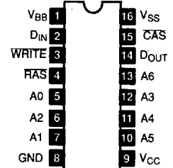
NTE2117 16-Lead DIP, See Diag. 249 NMOS, 16K Dynamic RAM (DRAM), 200ns
