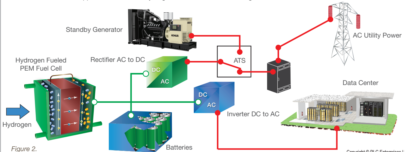
Data Center Application with PEM Hydrogen Fueled Fuel Cell Providing UPS Power to Data Center Critical Loads
