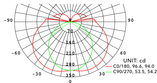
TGB-4-35-G1, 20Watts, 2600lm, Efficacy 130LPW, Beam Angle 120*
