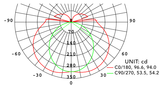
TGB-2-35-G1, 10Watts, 1300lm, Efficacy 130LPW, Beam Angle 120*
