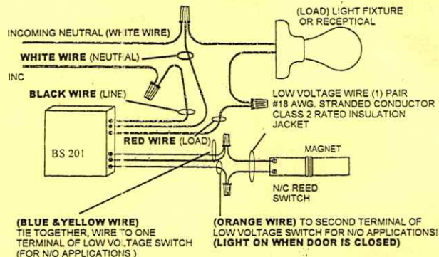
(BS-200 Series Diagram 1) BETTER SWITCH POWER CONTROLLER
