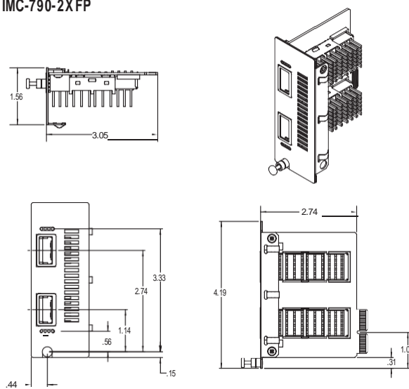
IMC-790-2XFP
