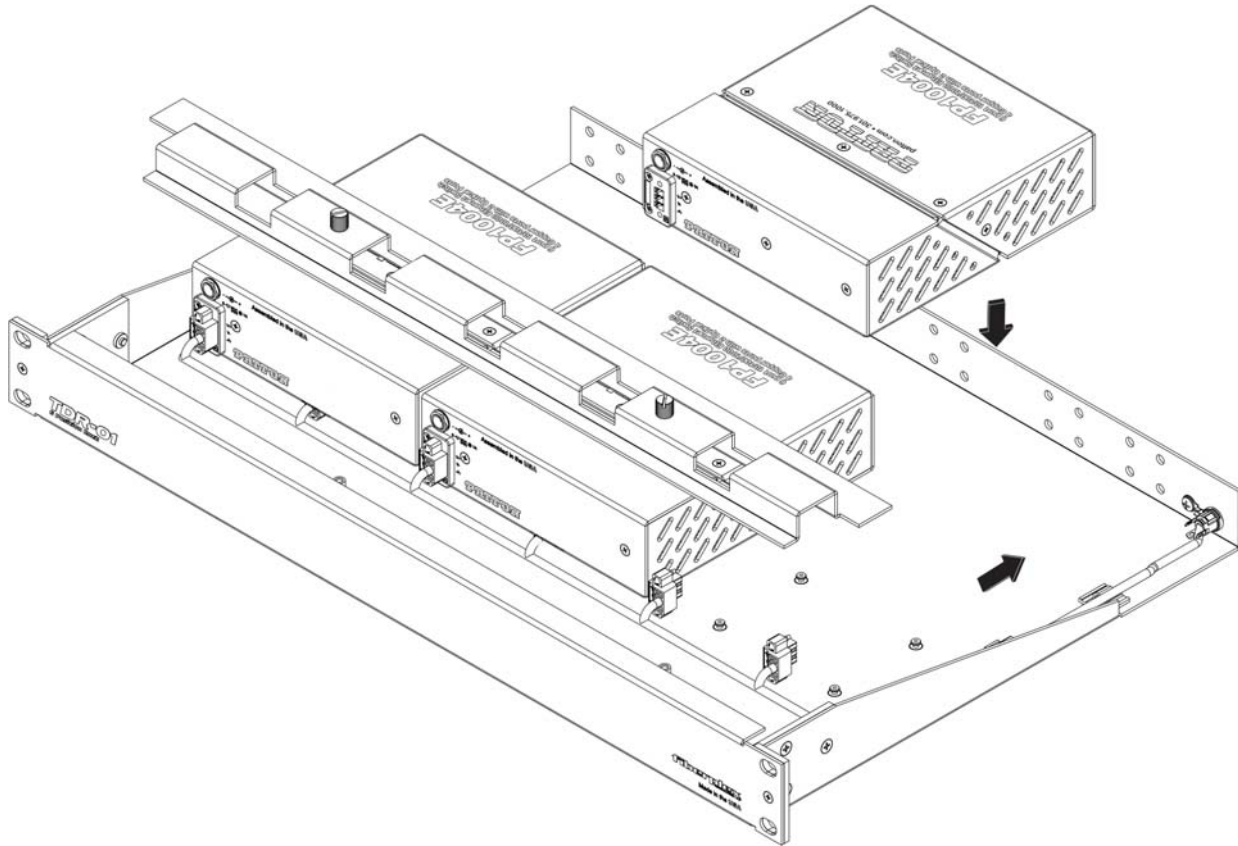
Figure 12. FP1004E installation on a TDR-01-AC tray
