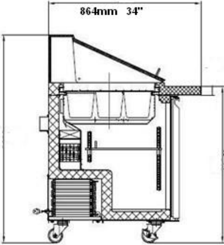
Section View
