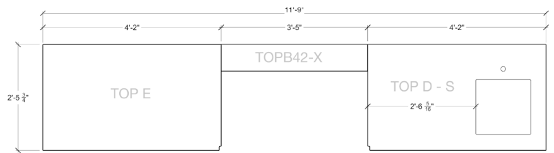
COUNTERTOP TEMPLATE
