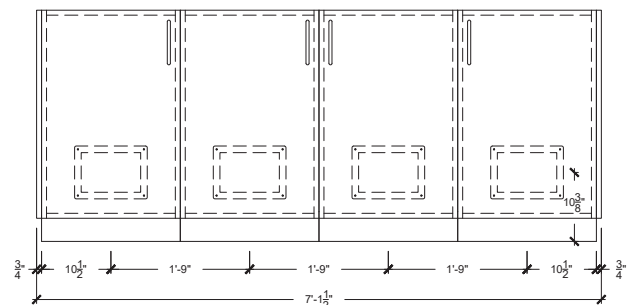
FRONT VIEW (Gas & Electrical Conduits Access Points)
