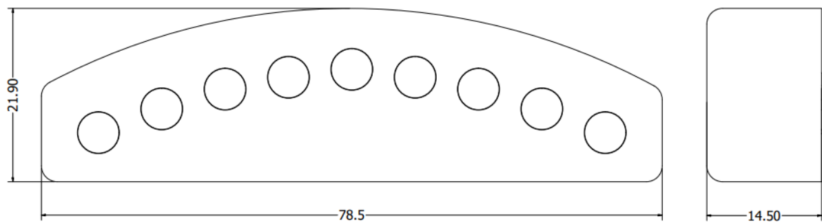
Fig.31 Overall dimensions
