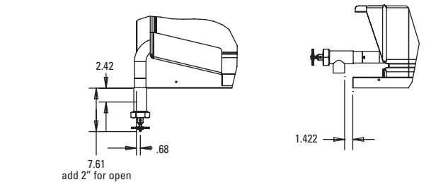
2" Draw-off valve – left side 90° front (BPD0V-3)
