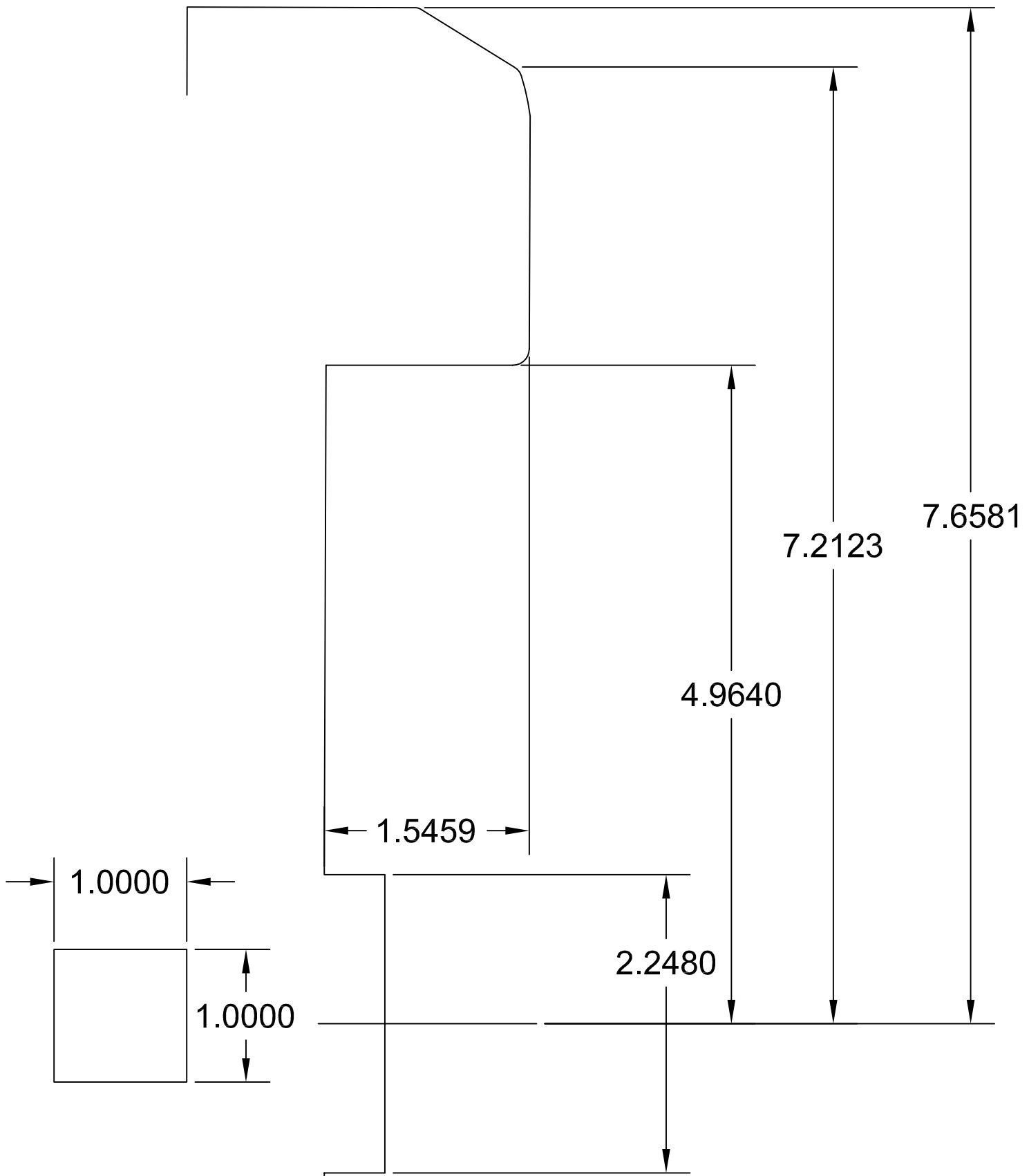
HPA Mk4 R32 355mm 6 Piston Brake System Wheel Clearance Template
