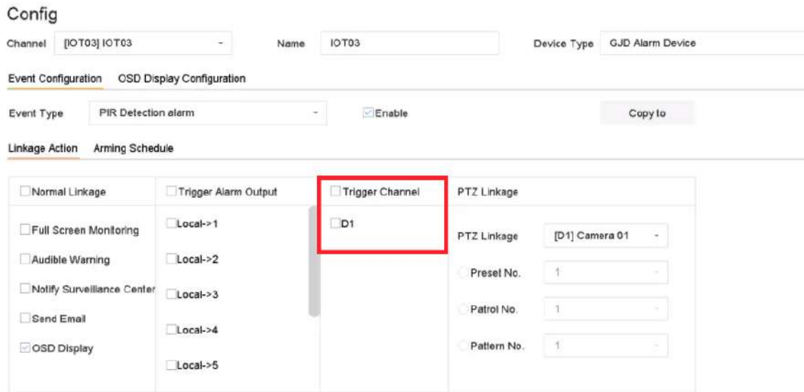
Figure 7-11 Trigger Channel
