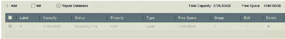
Figure 15-10 Repair Database
