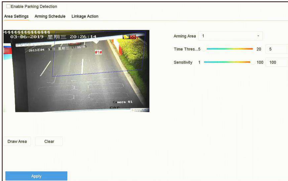
Figure 6-12 Parking Detection
