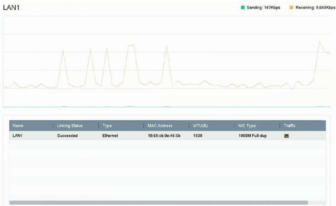
Figure 15-2 Network Traffic
