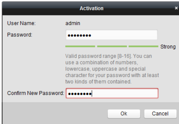
Figure 1-5 Activation
