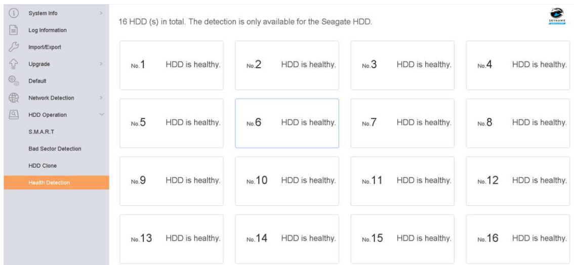
Figure 15-8 Health Detection
