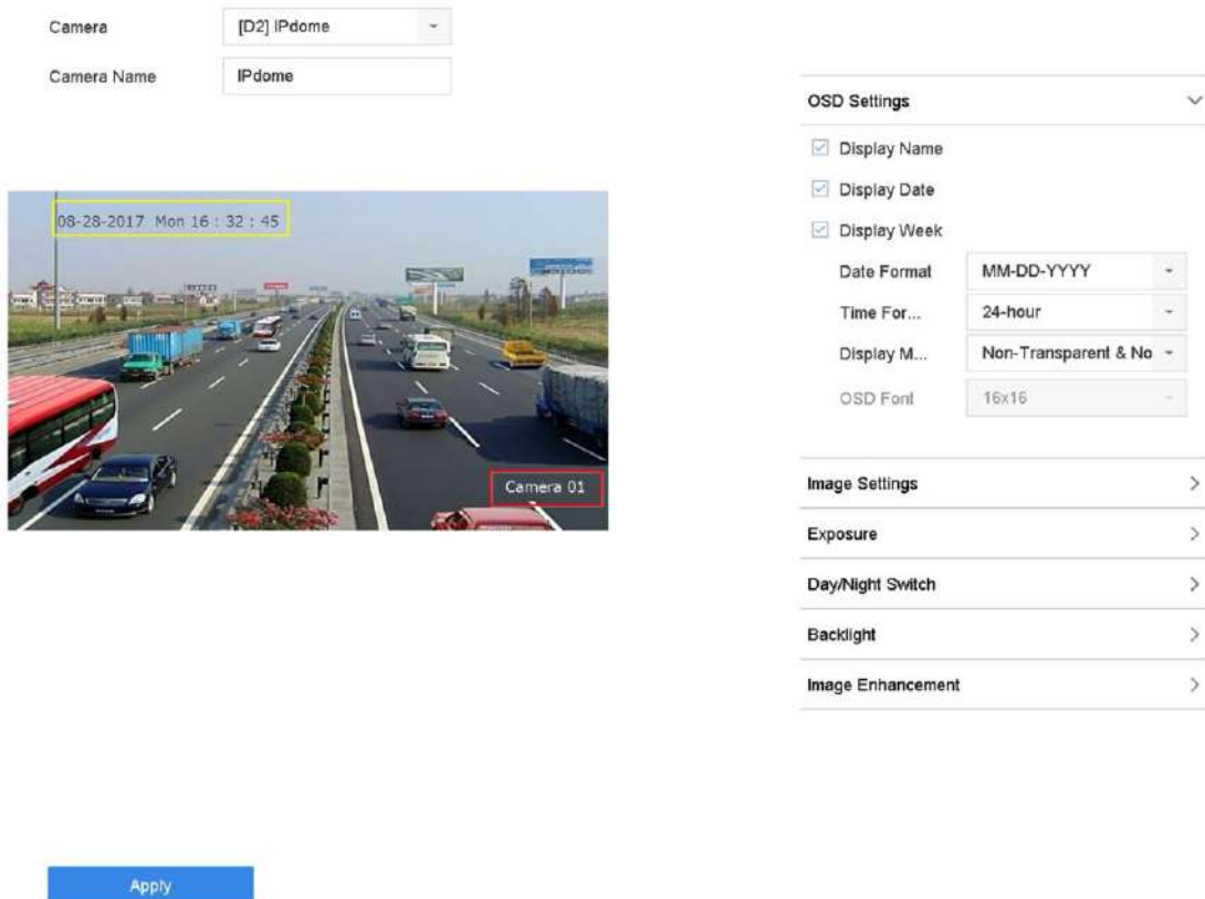
Figure 2-1 OSD Settings
