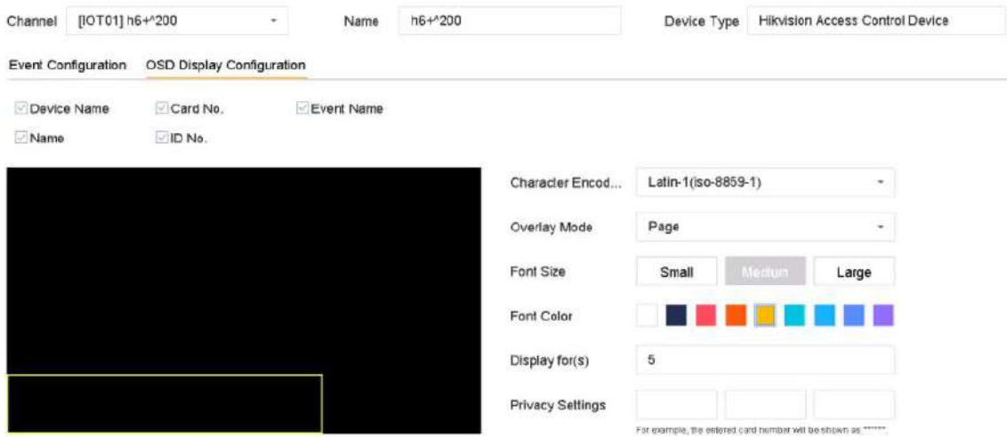
Figure 7-6 OSD Configuration
