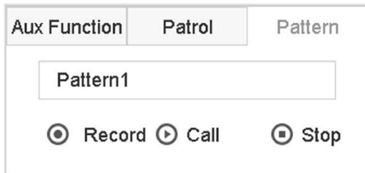
Figure 3-15 Pattern Configuration
