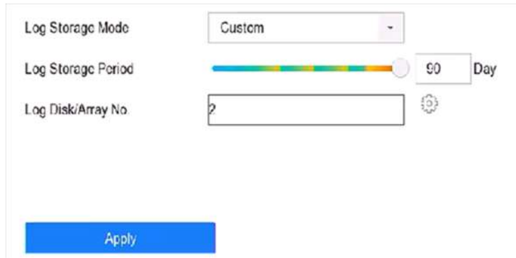
Figure 15-14 Log Storage
