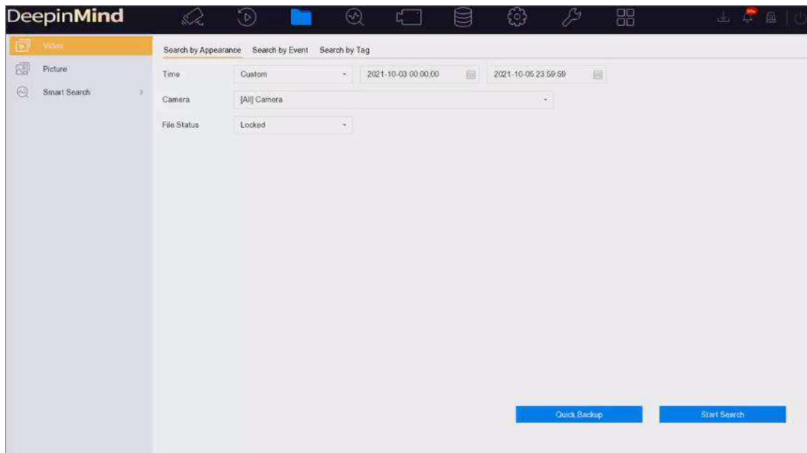
Figure 9-1 Quick Backup
