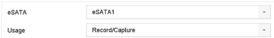
Figure 10-5 eSATA Mode
