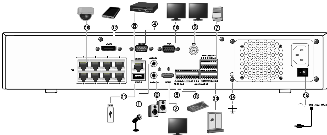
Figure 2: TVN 22S back panel connections
