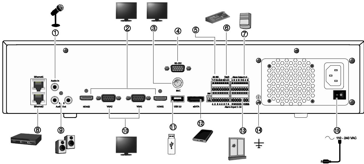
Figure 1: TVN 22P back panel connections
