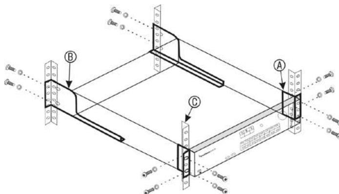
Figure 3: TVN 22S rack-mount installation
