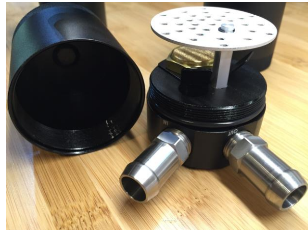
Inside view of catch can air deflector, baffle and filter
