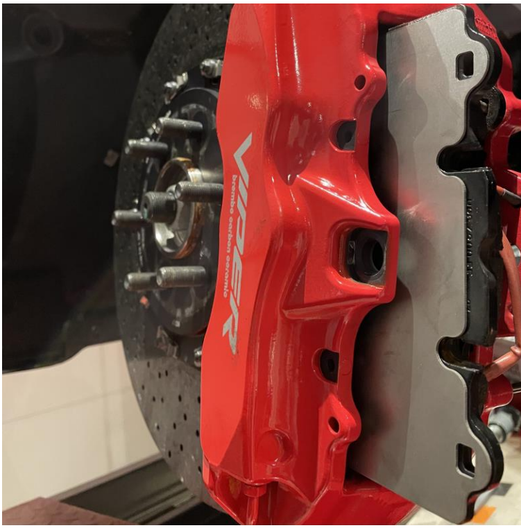
Installation of the Front (left) and Rear (right) Brake Pad Shields
