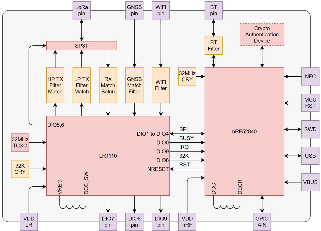
Figure 1 WM1110 Schematic diagram
