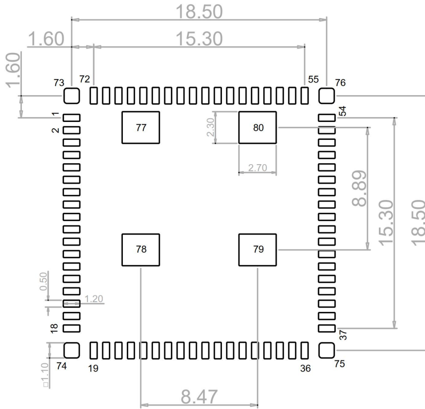
Figure 4 PCB Layout
