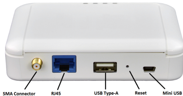
IoT Femto Gateway - I/O Ports
