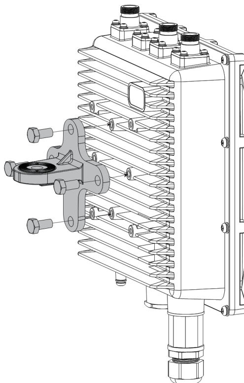
Figure 21: Mounting the cross bracket
