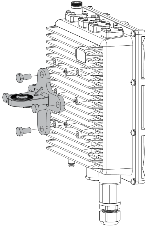
Figure 8: Mounting the cross bracket
