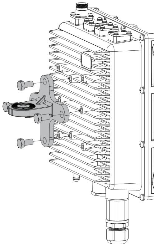
Figure 33: Mounting the cross bracket
