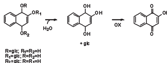
Scheme 1. Conversion of the three isomeric glucosides (hennosides) into the unique aglycone by hydrolysis in mildly acid conditions. Further transformation of the aglycone leads to the more stable lawsone by easy oxidation.
