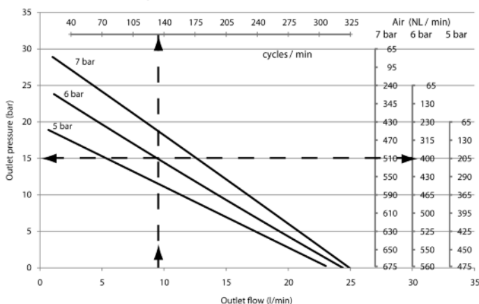
Pumpmaster 4 N.D. 5:1 HD SAE 30 23°C
