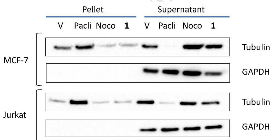
Figure 8. Compound 1 induces depolymerization of tubulin in vitro and in MCF-7 cells. A. Effect of compounds 1 and 7 on in vitro tubulin polymerisation. Purified bovine tubulin and GTP were mixed in a 96-well plate at 37 °C. Ethanol (1% v/v) was used as a vehicle control. The effect on tubulin assembly was monitored in a Spectramax 340PC spectrophotometer at 340 nm at 30 s intervals for 60 min at 37 °C. The results represent the mean for three separate
