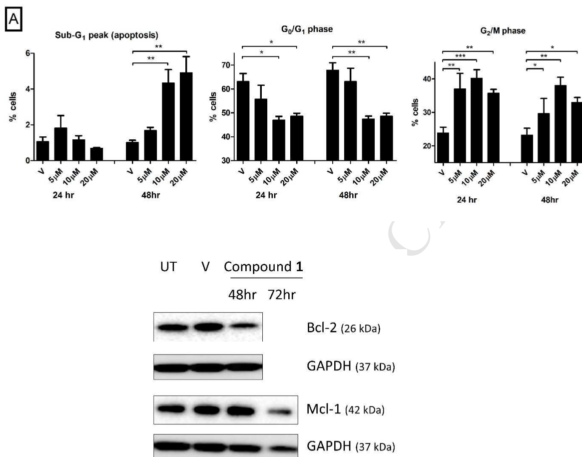
Figure 7.A. Effects of compound 1 on the cell cycle and apoptosis in MCF-7 cells. Cells were treated with either vehicle [V, 0.1% ethanol (v/v)], compound 1 (5, 10 or 20 \mu M) for 24 or 48 hr. Cells were then fixed, stained with PI, and analyzed by flow cytometry. Cell cycle analysis was performed on histograms of gated counts per DNA area (FL2-A). The number of cells with <2N (sub-G 1 ), 2N (G 0 G 1 ), and 4N (G 2 /M) DNA content was determined with CellQuest software. Values represent the mean \pm S.E.M. for three separate experiments. Statistical analysis was performed using one-way ANOVA followed by Dunnett's multiple comparison test; (*, p < 0.05 ; **, p < 0.01 ; ***, p < 0.001 ). B. Compound 1 downregulates the expression of anti-apoptotic proteins Bcl-2 and Mcl-1. MCF-7 cells were treated with 10 \mu M of compound 1. Untreated (UT) and vehicle (EtOH, 0.1 % v/v) controls were also examined. After the required
