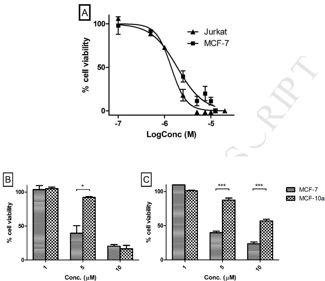
Figure 3A. Compound 1 decreases cell viability of Jurkat and MCF-7 cancer cells. Cells were grown in 96-well plates and treated with compound 1 at 0.1–20 μM for 48 h. Cell viability was expressed as a percentage of vehicle control [ethanol 1% (v/v)] and was measured by alamarBlue assay (average of three independent experiments). Figure 3B, C. Effects of compounds 7 and 13 on the viability of MCF10a human mammary epithelial cells. Cells were treated with compound 7 (B) or 13 (C) (1, 5, 10 and 20 μM) for 48 hr. Cell viability was expressed as a percentage of vehicle control [ethanol 1% (v/v)] and was measured by alamarBlue assay (average of three independent experiments). A non-paired two-tailed t-test was used to test for statistical significance (*, p < 0.05 ; ***, p < 0.001 )
