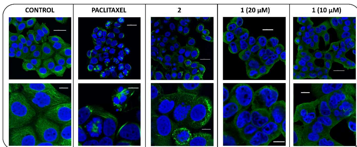
Figure 9. Compound 1 depolymerises the microtubule network of MCF-7 breast cancer cells. Cells were treated with vehicle control [1% ethanol (v/v)], paclitaxel (1 \mu\text{M} ), compound 2 (100 nM) or compound 1 (10 or 20 \mu\text{M} ) for 16 h. Cells were fixed in 4% paraformaldehyde and stained with mouse monoclonal anti- \alpha -tubulin-FITC antibody (clone DM1A) (green), Alexa Fluor 488 dye and counterstained with DAPI (blue). Images were captured by Leica SP8 confocal microscopy with Leica application suite X software. Representative confocal micrographs of three separate experiments are shown. Scale bar: 30 \mu\text{M} (top images); 10 \mu\text{M} (bottom images).
