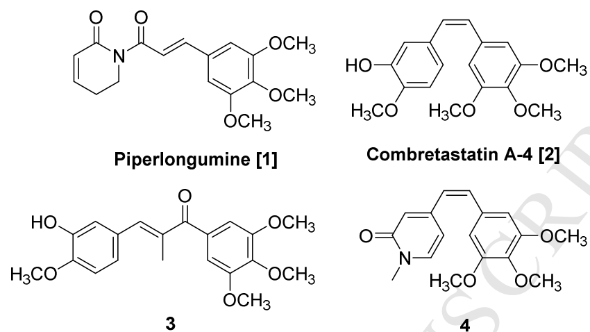
Figure 1. Structures of piperlongumine, combretastatin A-4 and analogues.
