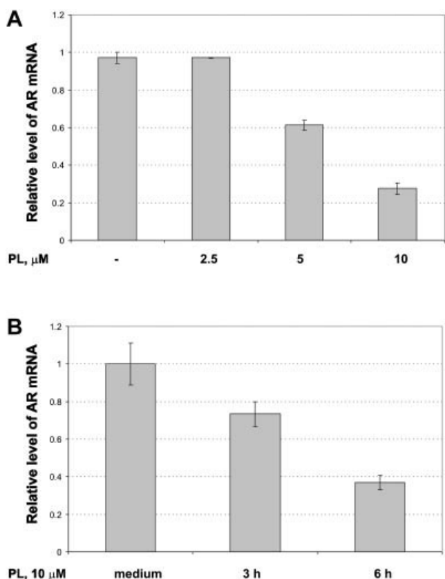
Fig. 3. Levels of AR mRNA in LNCaP cells treated with PL. A: Cells were treated with indicated concentrations of PL. AR mRNA levels were detected by Real Time PCR using specific primers. B: Cells were treated with PL (10 \mu M) for the indicated periods of time. AR mRNA levels were detected by Real Time PCR.
