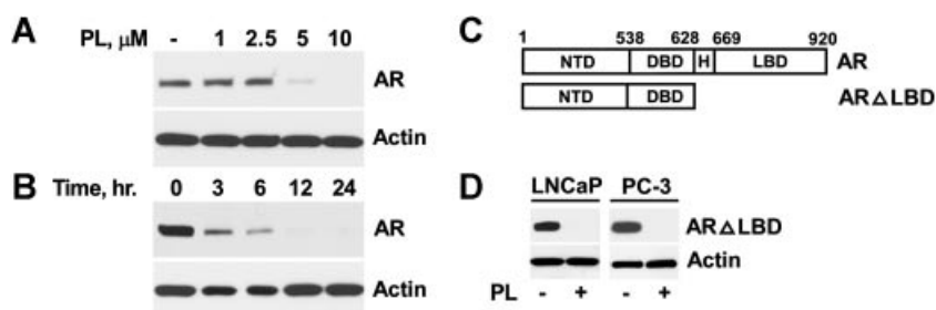
Fig. 2. PL down-regulates the expression of AR in prostate cancer cells. A: PL induces dose-dependent reduction of AR protein levels in LNCaP cells. Cells were treated with PL for 3 hr. Cell lysates were subjected to SDS-PAGE, blotted, and probed with specific antibodies. B: Time course of AR protein depletion in LNCaP cells treated with PL (10 \mu M). Cells were cultured in the presence of PL for the indicated periods of time. Expression of AR and actin was detected by immunoblotting with anti-AR or anti-actin antibodies, respectively. C: Structural domains of full length human AR and AR \Delta LBD. D: LNCaP and PC-3 prostate cancer cells were transfected with a plasmid encoding AR \Delta LBD. Cells were treated with PL (10 \mu M) for 3 hr. Expression of AR \Delta LBD was examined by western blot analysis.
