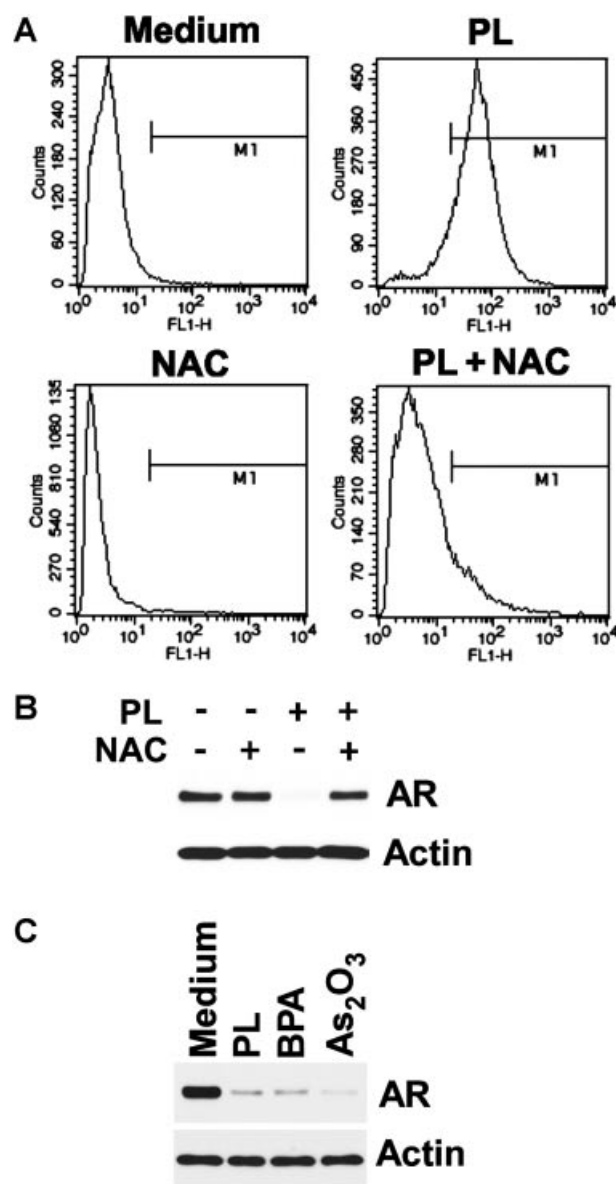
Fig. 6. PL reduces AR protein levels via ROS-dependent mechanism. A: PL induces ROS production in LNCaP cells. LNCaP cells were treated with PL (10 \mu\text{M} ) with or w/o NAC (5 mM) for 1 hr, stained with CM-H 2 DCFDA and analyzed by flow cytometry as described in Materials and Methods section. B: Cells were treated with PL (10 \mu\text{M} ) with or w/o NAC (5 mM) for 3 hr. Expression of AR and actin was detected by immunoblotting with anti-AR and anti-actin antibodies, respectively. C: Cells were treated with PL (10 \mu\text{M} ), bisphenol A (100 \mu\text{M} ), or arsenic (III) oxide (25 \mu\text{M} ) for 3 hr. Expression of AR and actin was detected by immunoblotting with anti-AR and anti-actin antibodies, respectively.
