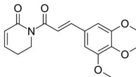
Fig. 1. Chemical structure of PL molecule.
