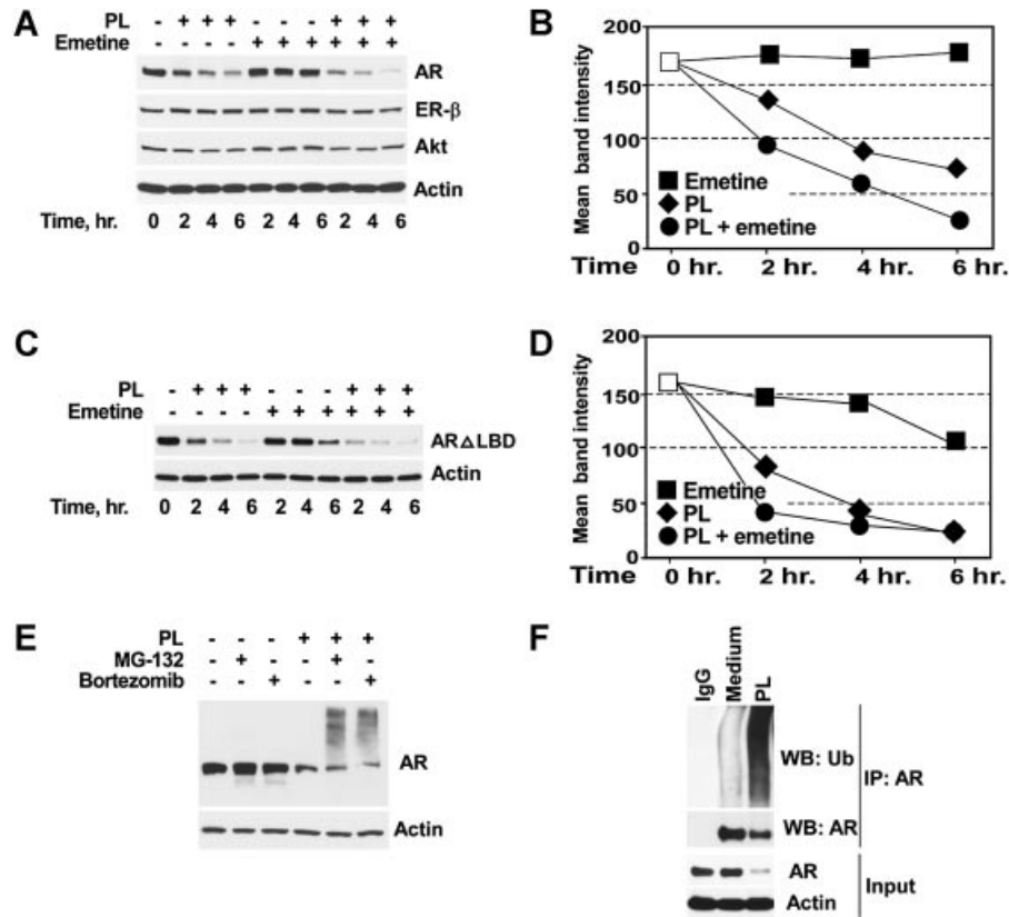
Fig. 4. PL induces depletion of AR at post-transcriptional level. A: AR protein levels were determined by Western blot analysis after incubation of LNCaP cells with PL (10 \mu M) with or w/o emetine (10 \mu M) for the indicated periods of time. B: Densitometry readings of the immunoblot shown in panel A. The intensity of the signal was quantitated by ImageJ 1.45i software. C: PC-3 cells transfected with AR \Delta LBD vector were incubated with PL (10 \mu M) with or w/o emetine (10 \mu M) for the indicated periods of time. Protein levels were determined by western blot analysis. D: Densitometry readings of the immunoblot shown in panel C. The intensity of the signal was quantitated by ImageJ 1.45i software. E: Co-treatment with proteasomal inhibitors, MG-132 and bortezomib, induces accumulation of slow-migrating ubiquitinated forms of AR in PL-treated LNCaP cells. Cells were treated with PL (10 \mu M) with or w/o MG-132 (10 \mu M) or bortezomib (10 \mu M) for 3 hr. Expression of AR and actin was detected by immunoblotting with anti-AR or anti-actin antibodies, respectively. F: LNCaP cells were treated with PL (10 \mu M) for 3 hr. Cell lysates were subjected to IP with antibodies to AR followed by western blot analysis using antibody to ubiquitin. Aliquots of cell lysates (Input) were also subjected to western blot analysis.
