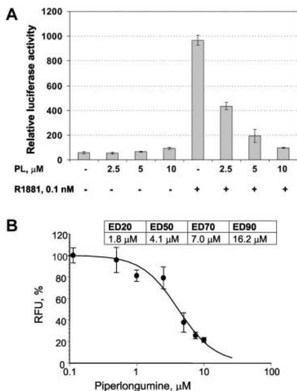
Fig. 5. PL attenuates the transcriptional activity of the AR and suppresses proliferation of LNCaP cells. A: Analysis of transcriptional activity was performed as described in Materials and Methods section. Columns, means of three different experiments; bars, SDs. B: LNCaP cells cultured in the presence of escalating concentrations of PL for 48 hr. The effect of PL on cellular proliferation was analyzed by CellTiter Blue assay. EDs were calculated as described in Materials and Methods section.
