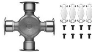
Cruceta Medida 5-170X 2 3/8"
