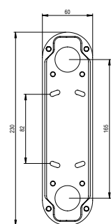
WALL PLATE
