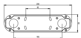
CEILING PLATE
