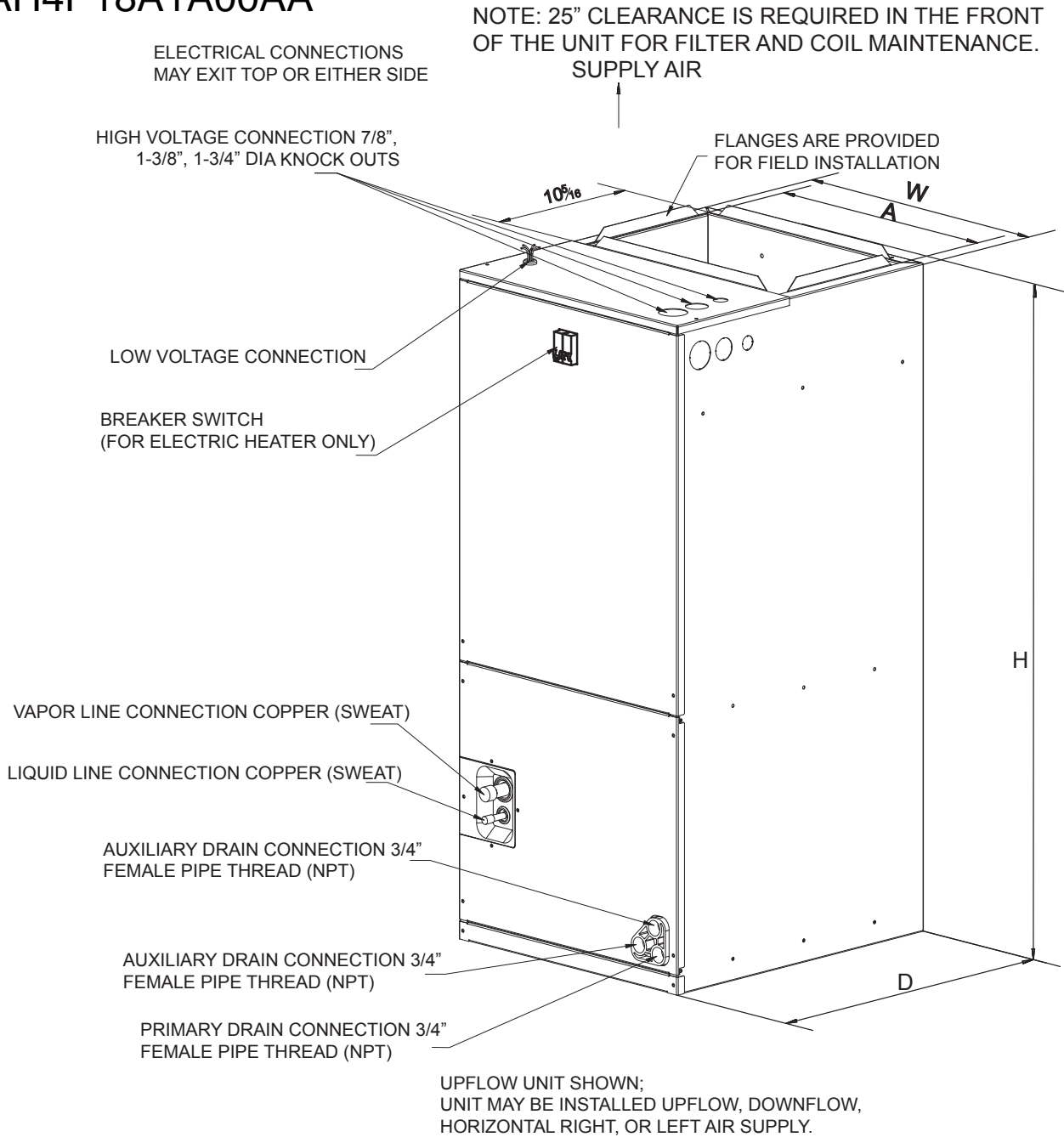
Fig.1 DIMENSIONS
