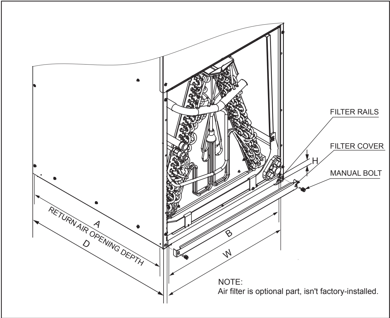
Fig.2 EXTERNAL FILTER BASE
