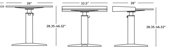
OE1 Sit-to-Stand Table - Rectangular with Wrap
