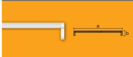
Box Type Luminaire for LED T8 Tube (Single-Ended)
