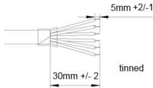
Figure 4-2 USBC-FS-UART-5V-5V-1800-WE Mechanical Details (dimensions in mm)
