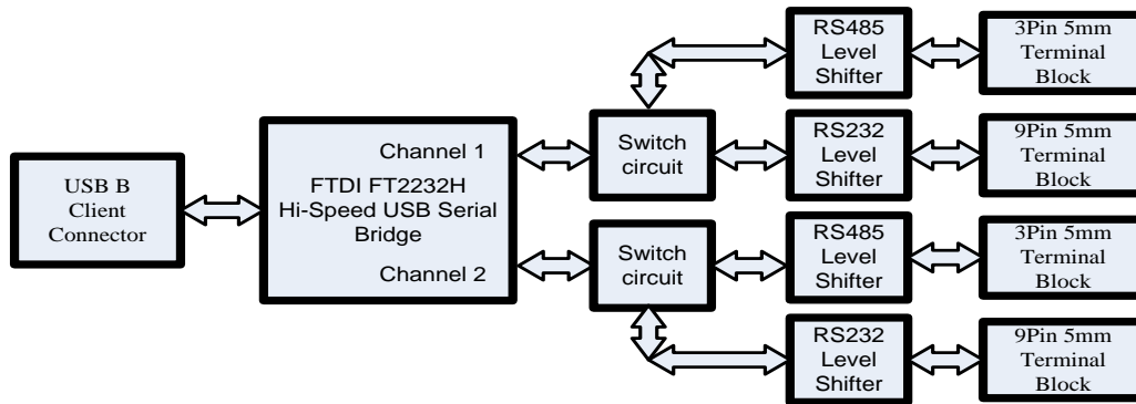
Figure 1.2 USB2-H-9002-M Block Diagram
