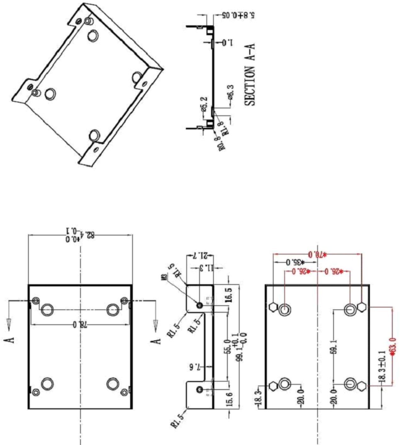
Figure 5.2 USB2-H-9002-M Case Dimensions - Bottom
