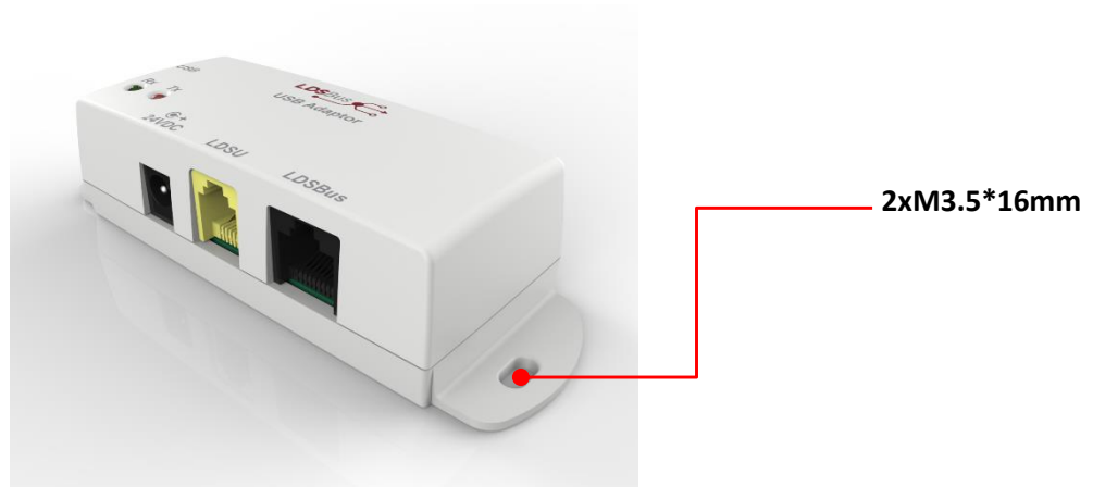
Figure 4 – LDSBus USB Adapter Flush Mount
