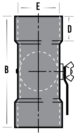
STANDARD WINDGATE
