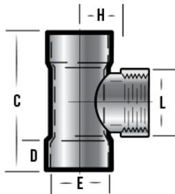
ADAPTER TEE
