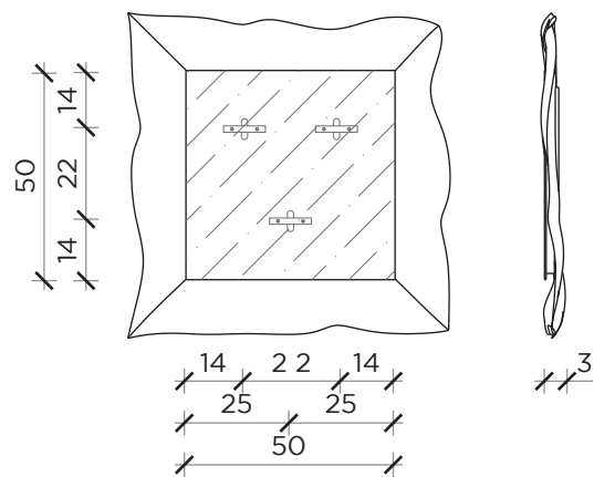
FRONTE | FRONT
