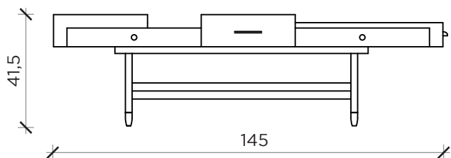
FRONTE | FRONT
